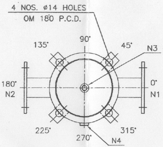
NOZZLE ORIENTATION
