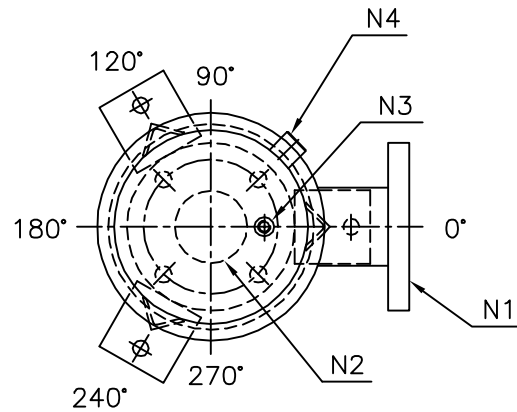
NOZZLE ORIENTATION
