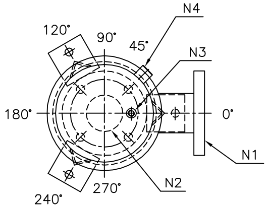
NOZZLE ORIENTATION
