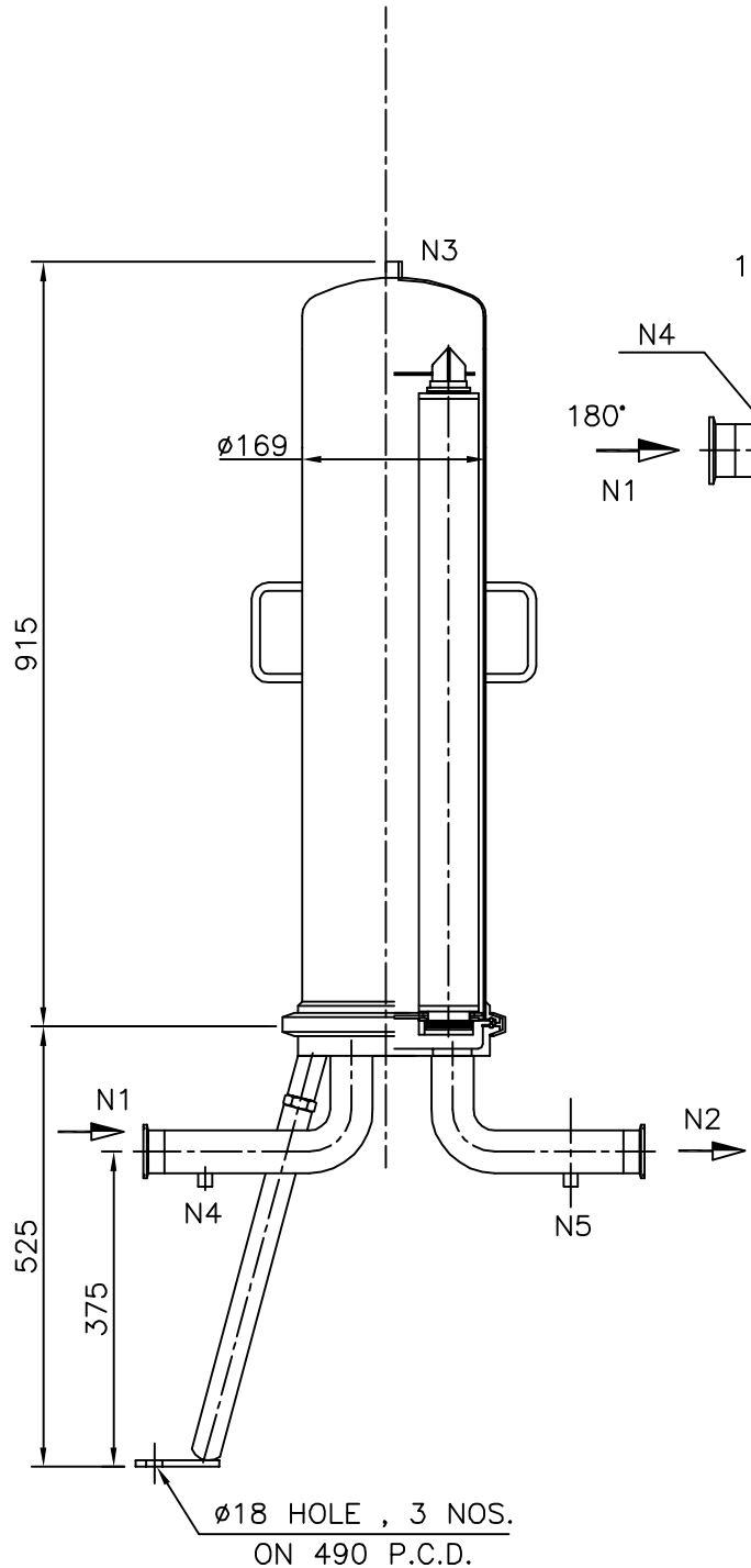
NOZZLE ORIENTATION
