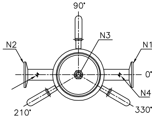
NOZZLE ORIENTATION
