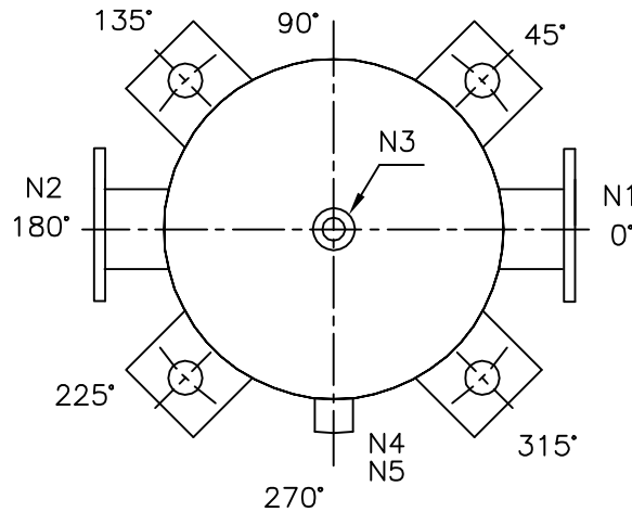
NOZZLE ORIENTATION
