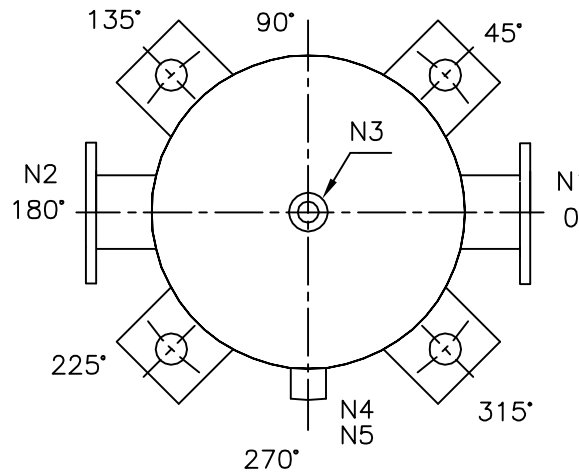
NOZZLE ORIENTATION
