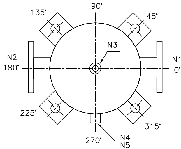
NOZZLE ORIENTATION
