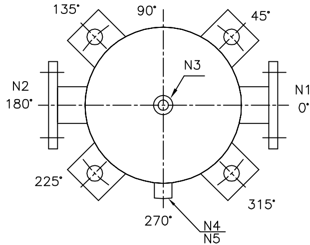
NOZZLE ORIENTATION
