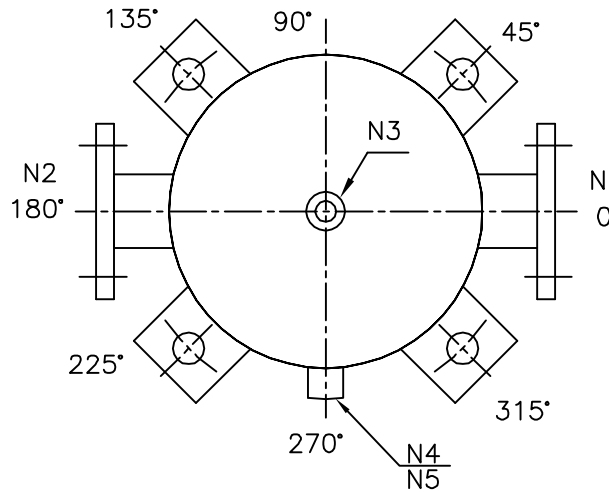
NOZZLE ORIENTATION
