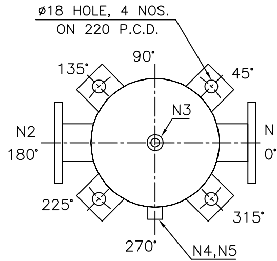
NOZZLE ORIENTATION
